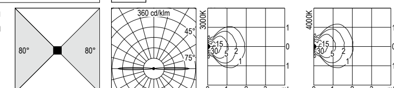
5373.GVX.T.-- 20 W 1+1 Led 3000 K 2 x 720 lm 5373.GZX.T.-- 20 W 1+1 Led 4000 K 2 x 750 lm 220-240 V 50/60 HZ vetro trasparente clear diffuser alimentatore incluso led driver integral
